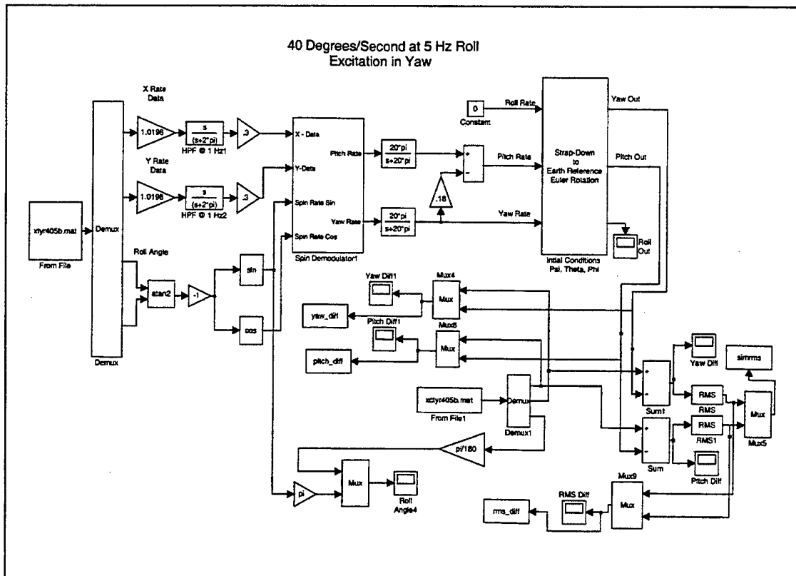
Figure 20. Euler Rotation Model For 40 Degrees/Second 5Hz Data With Roll Reference Provided From The Roll Sensor. Model RMPTYR405B.MDL.
